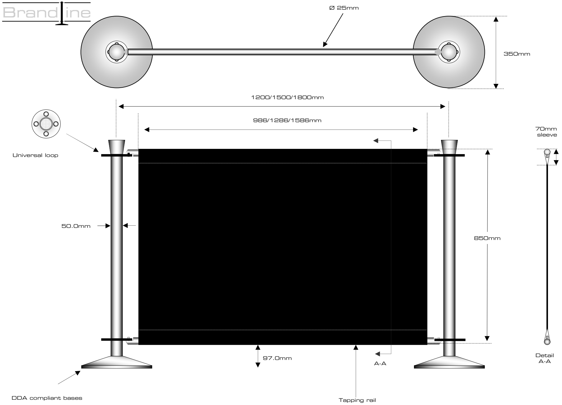
Brandline™ barrier system - dimensional data
