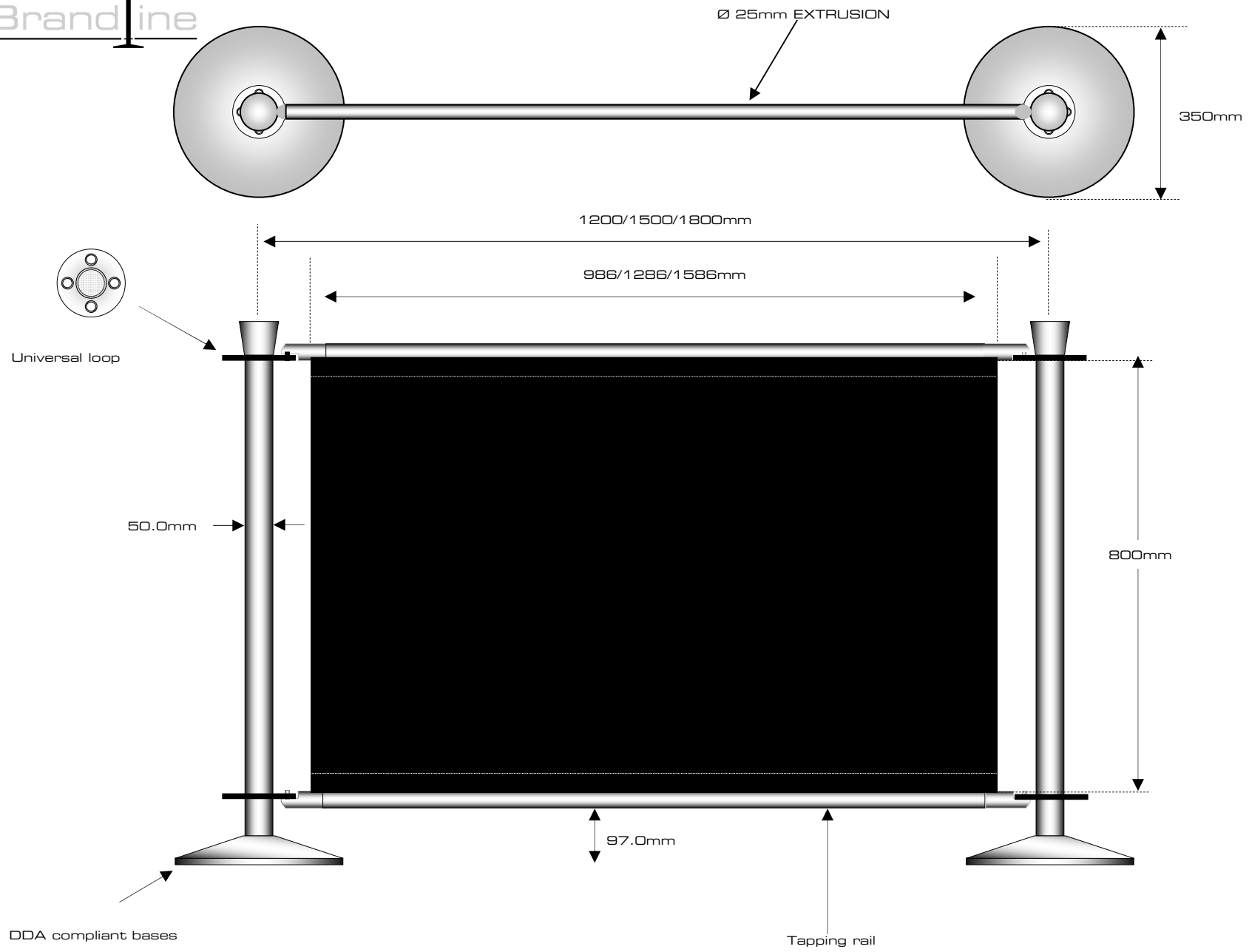
Brandline™ barrier system - dimensional data
